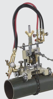
MANUAL GAS PIPE CUTTER
